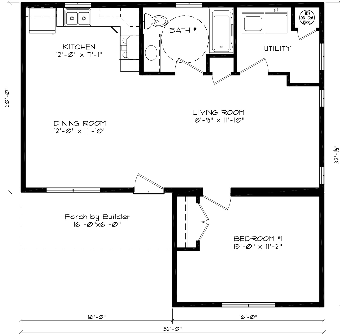
COTTAGE #4 32' x 20' / 32' 832 SQ. FT.
